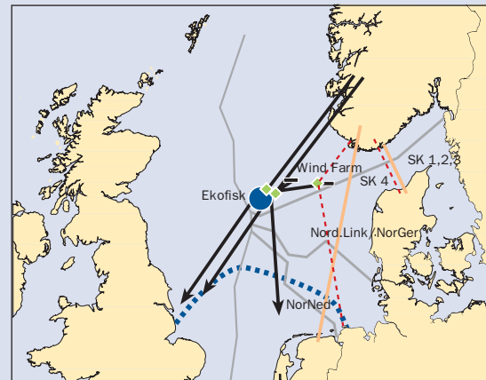
Figure S.8: Offshore grid proposal by Statnett
