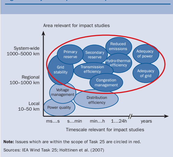
Figure S.6: System impacts of wind power
