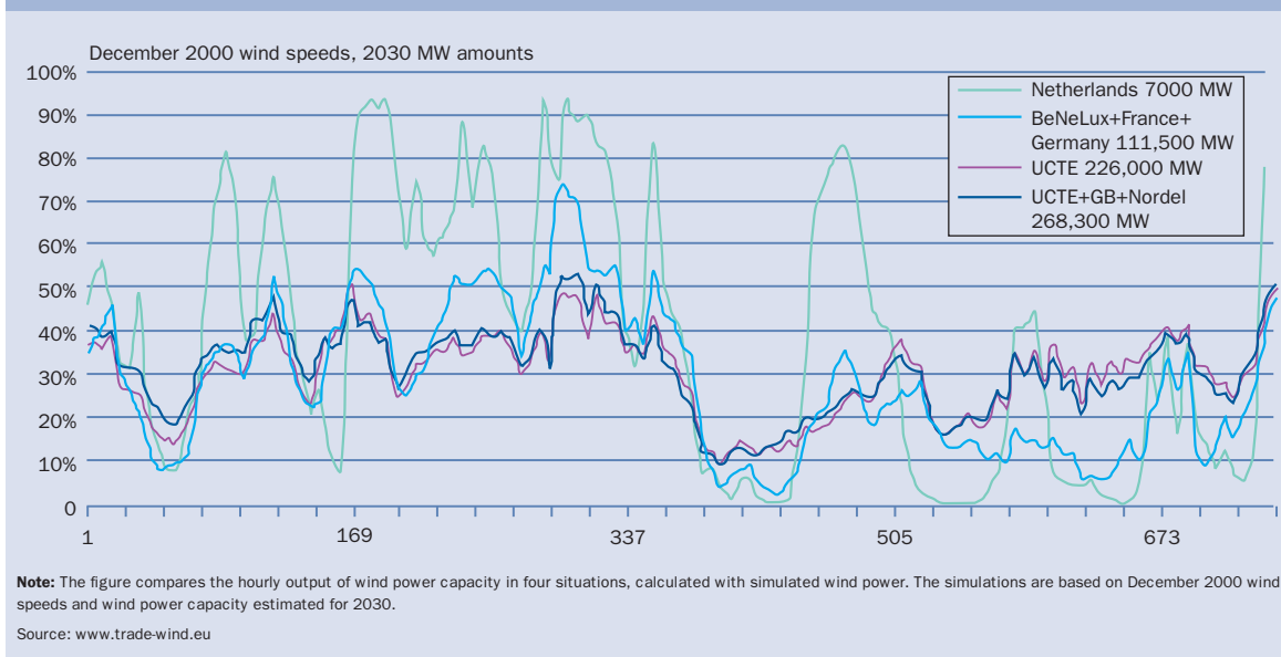
Figure S.5: Example of smoothing effect by geographical dispersion
