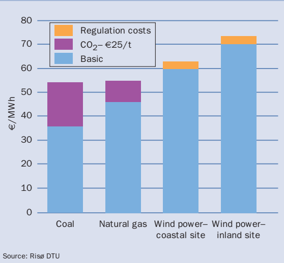
Figure S.14: Costs of generated power comparing conventional plants to wind power, 2010 (constant 2006-€)
