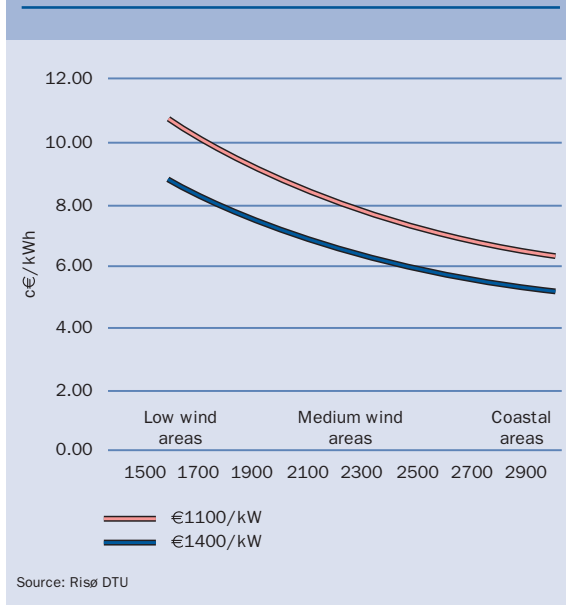
Figure S.11: Calculated costs per kWh of wind generated power as a function of the wind regime at the chosen site (number of full load hours)
