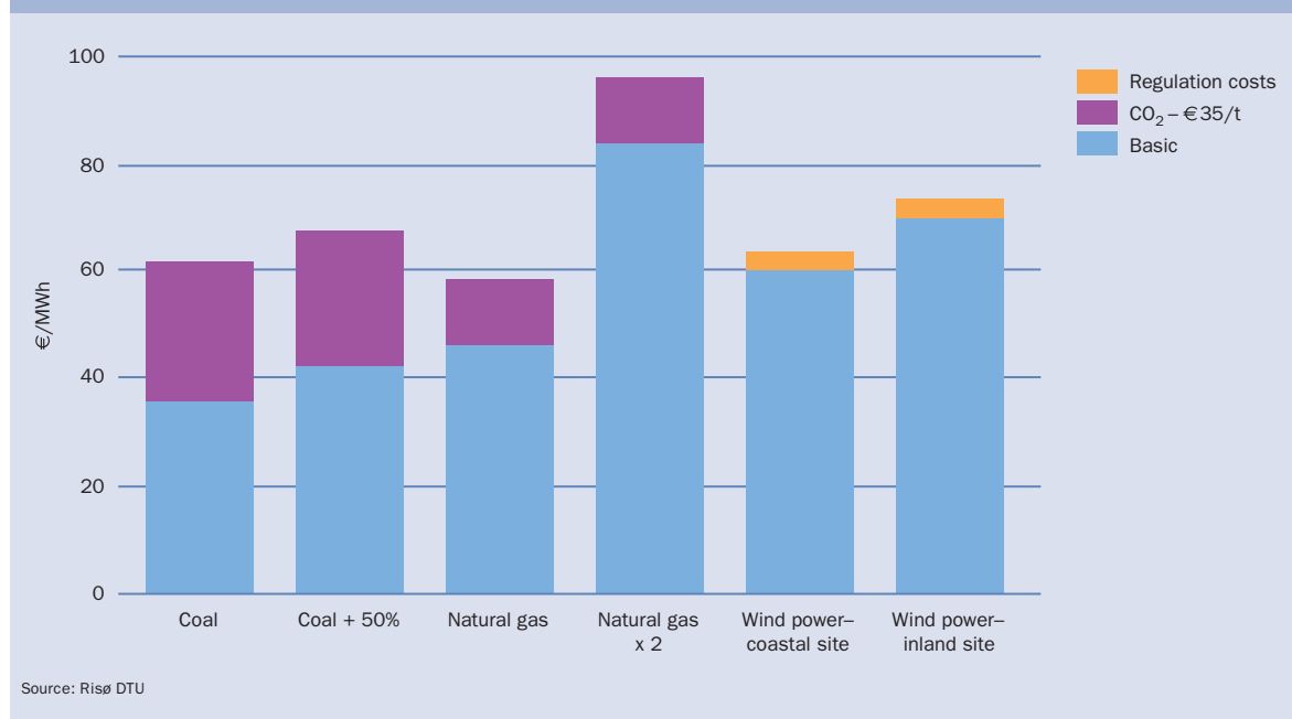
Figure S.15: Sensitivity analysis of costs of generated power comparing conventional plants to wind power, assuming increasing fossil fuel and CO 2 prices, 2010 (constant 2006-€)
