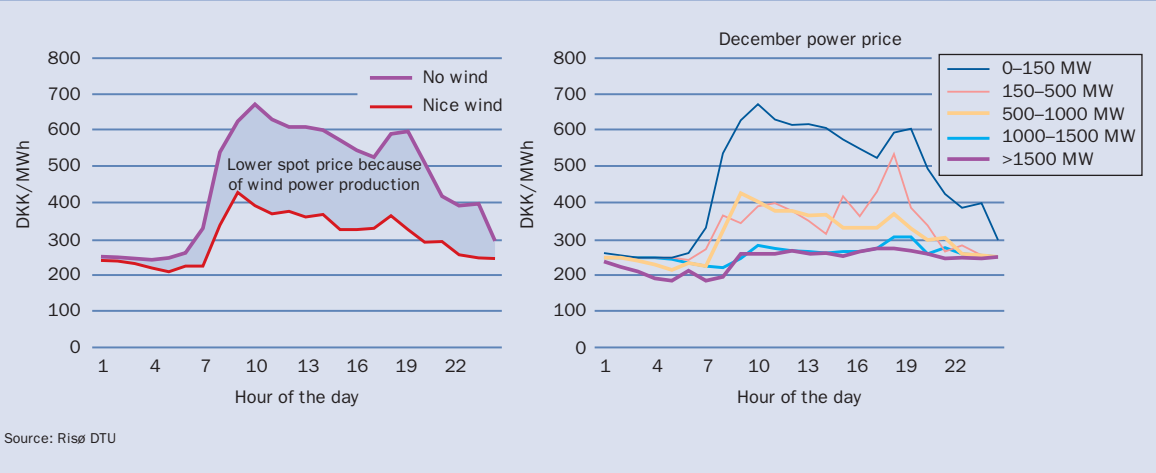
Figure S.13: The impact of wind power on the spot power price in the West Denmark power system in December 2005
