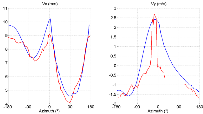
Fig. 2 Induced wind speed along the blades path at hub height 27 m.
